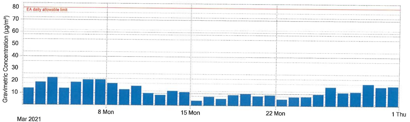
Figure 1: Jondaryan Township TSP continuous monitoring 24 Hr average results for March 2021
