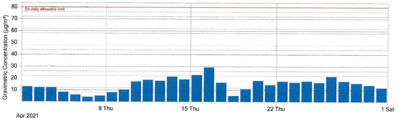
Figure 1: Jondaryan Township TSP continuous monitoring 24 Hr average results for April 2021
