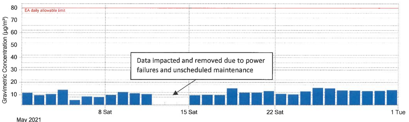
Figure 1: Jondaryan Township TSP continuous monitoring 24 Hr average results for May 2021
