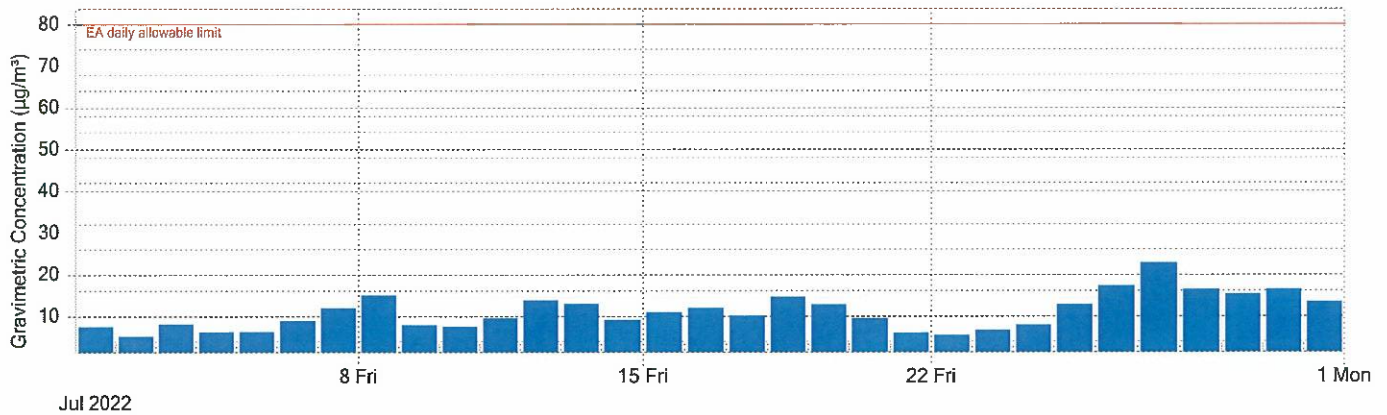
Figure 1: Jondaryan Township TSP continuous monitoring 24 Hr average results for July 2022
